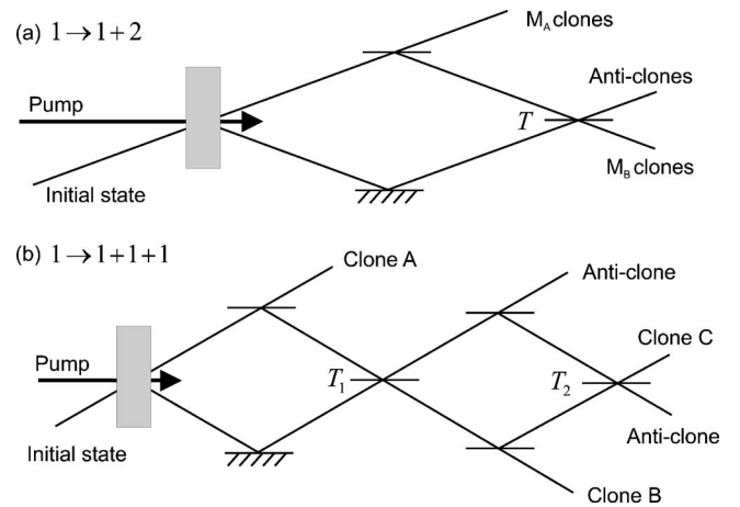
FIG. 1. Optical implementation of (a) the 1 \rightarrow 1+2 and (b) the 1 \rightarrow 1+1+1 optimal asymmetric cloning machines.
